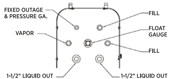
FITTING LAYOUT UNDER FITTING COVER
